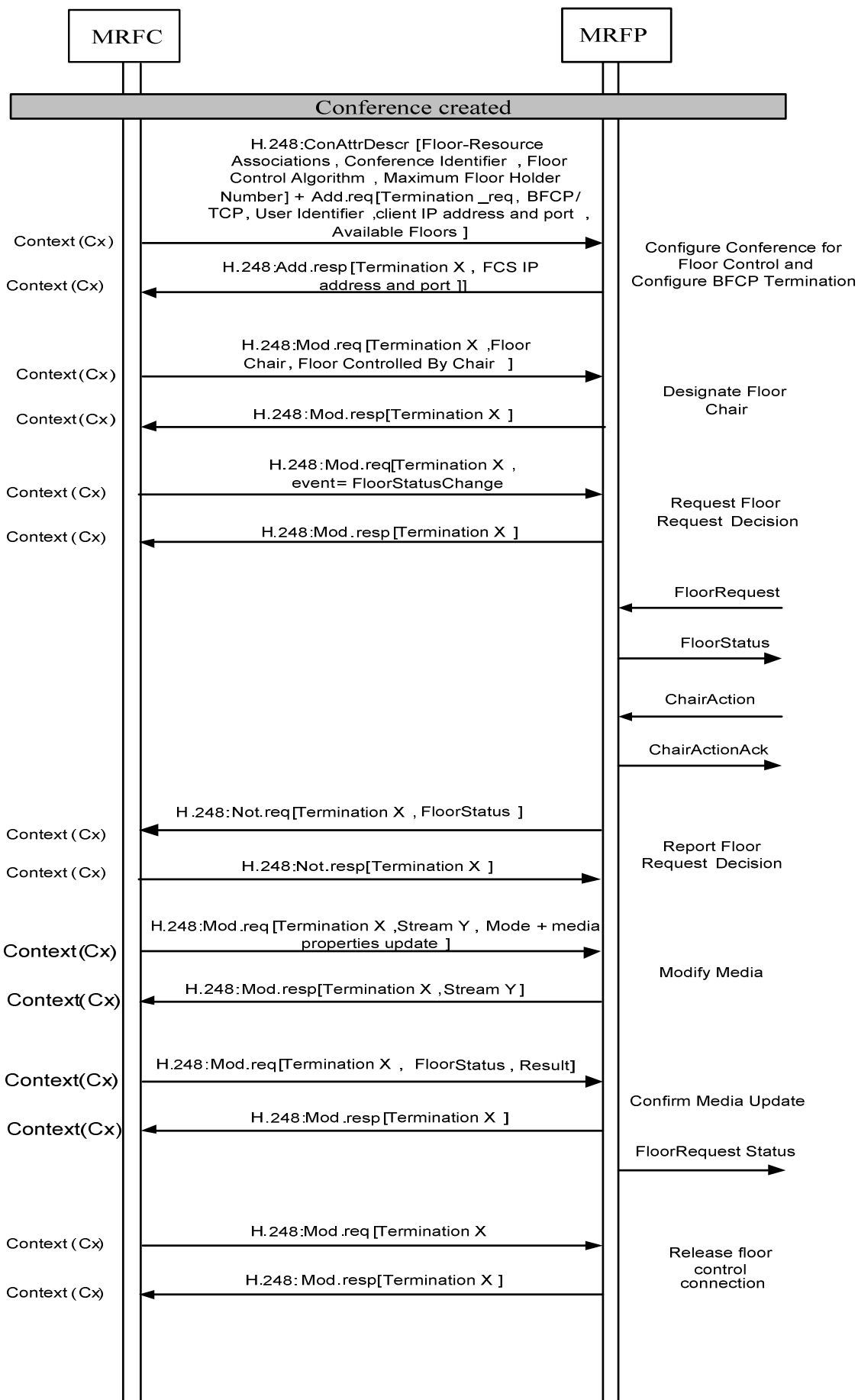
Figure 6.2.13.1 Floor control (message sequence chart)
