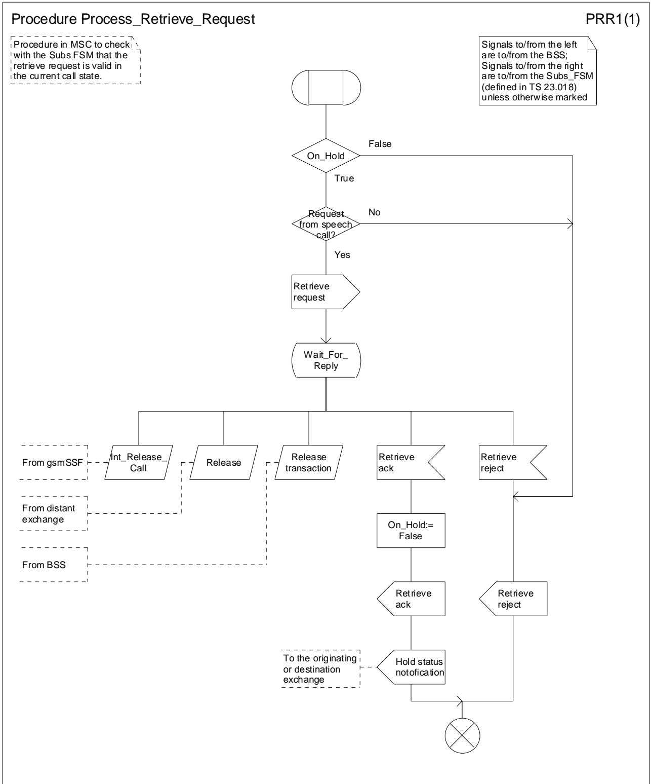
Figure 2.2b: Procedure Process_Retrieve_Request
